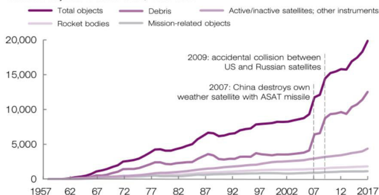
Tracked objects in Earth orbit, 1957-2017
